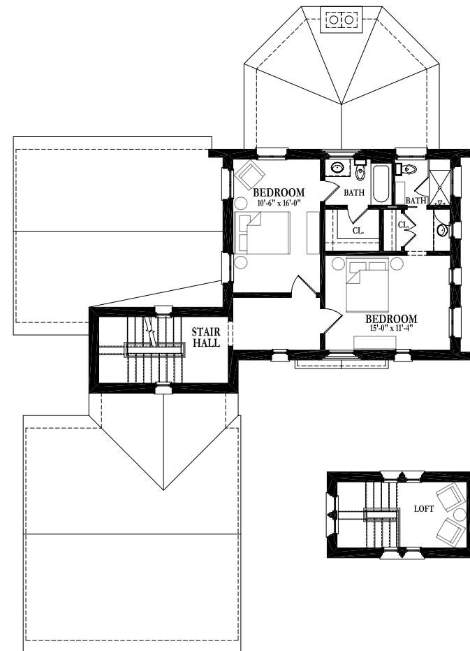
UPPER LEVEL & LOFT PLAN
